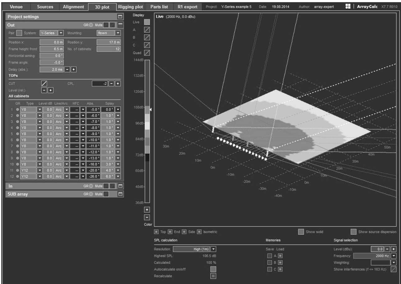
Y-Series setup example 5, 3D plot: Outer arrays 10 x Y8 + 2 x Y12, inner arrays 10 x Y8, 32 Y-Sub SUB array
