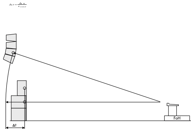
Time alignment of ground stacked cabinets
