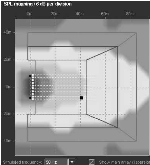
50 Hz mapping of 10 delay-arc'd omnidirectional subwoofers
