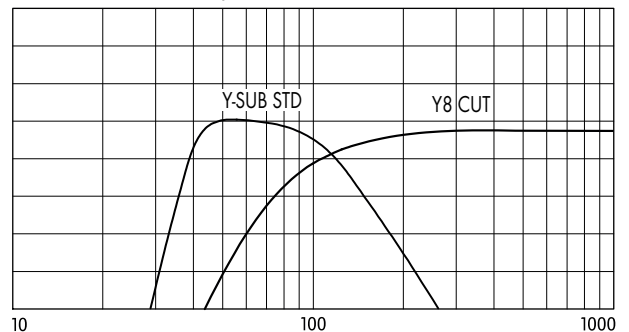
Y8 / Y-SUB / J-SUB crossover setup
