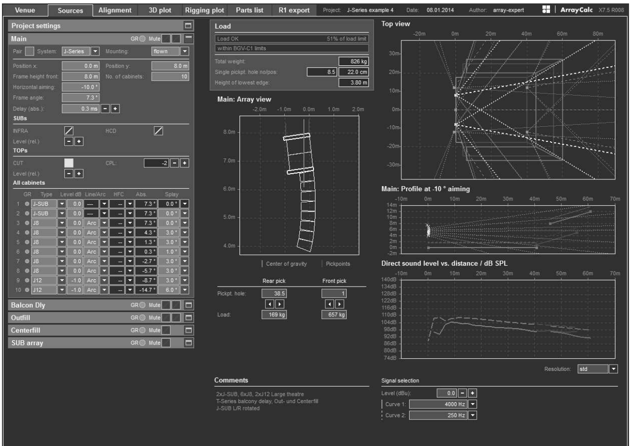
J-Series setup example 4, Arrays: Large theater 2 x J-SUB, 6 x J8, 2 x J12 ; T-Series balcony delay, Outfill and Centerfill; J-SUB L/R rotated
