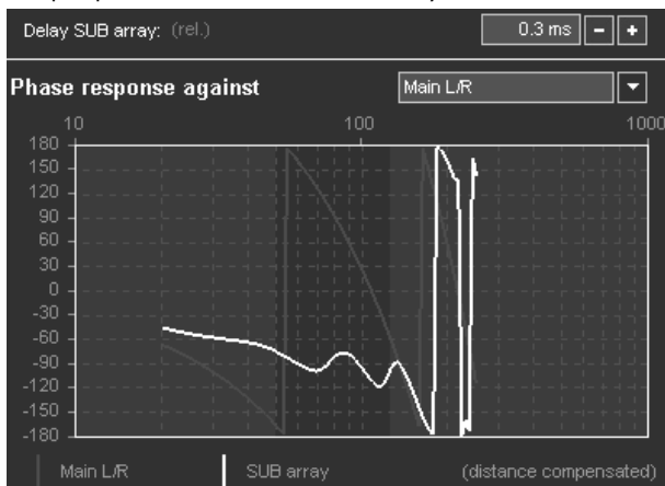
Phase response - not aligned
