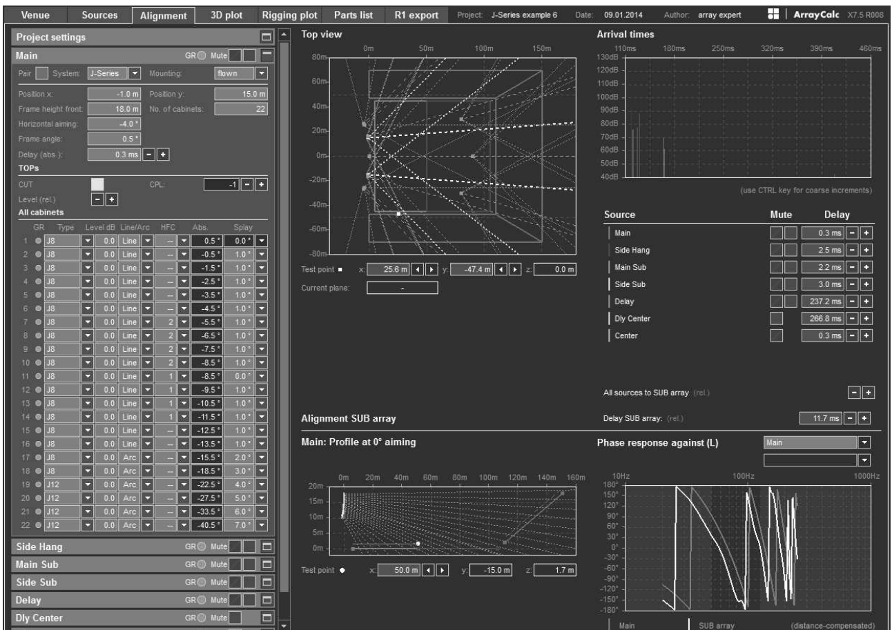
J-Series setup example 6, Alignment: Stadium setup
