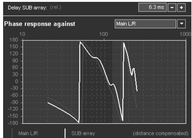
Phase response - correctly aligned
