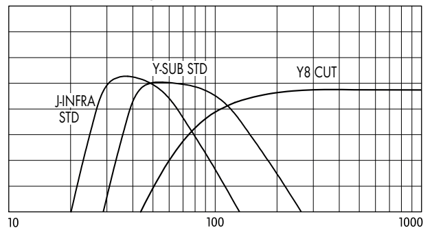
Y8 / Y-SUB / J-INFRA crossover setup
