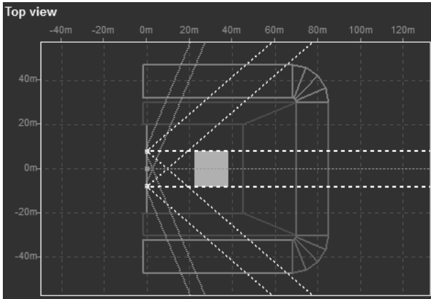
Top view of listening planes and arrays
